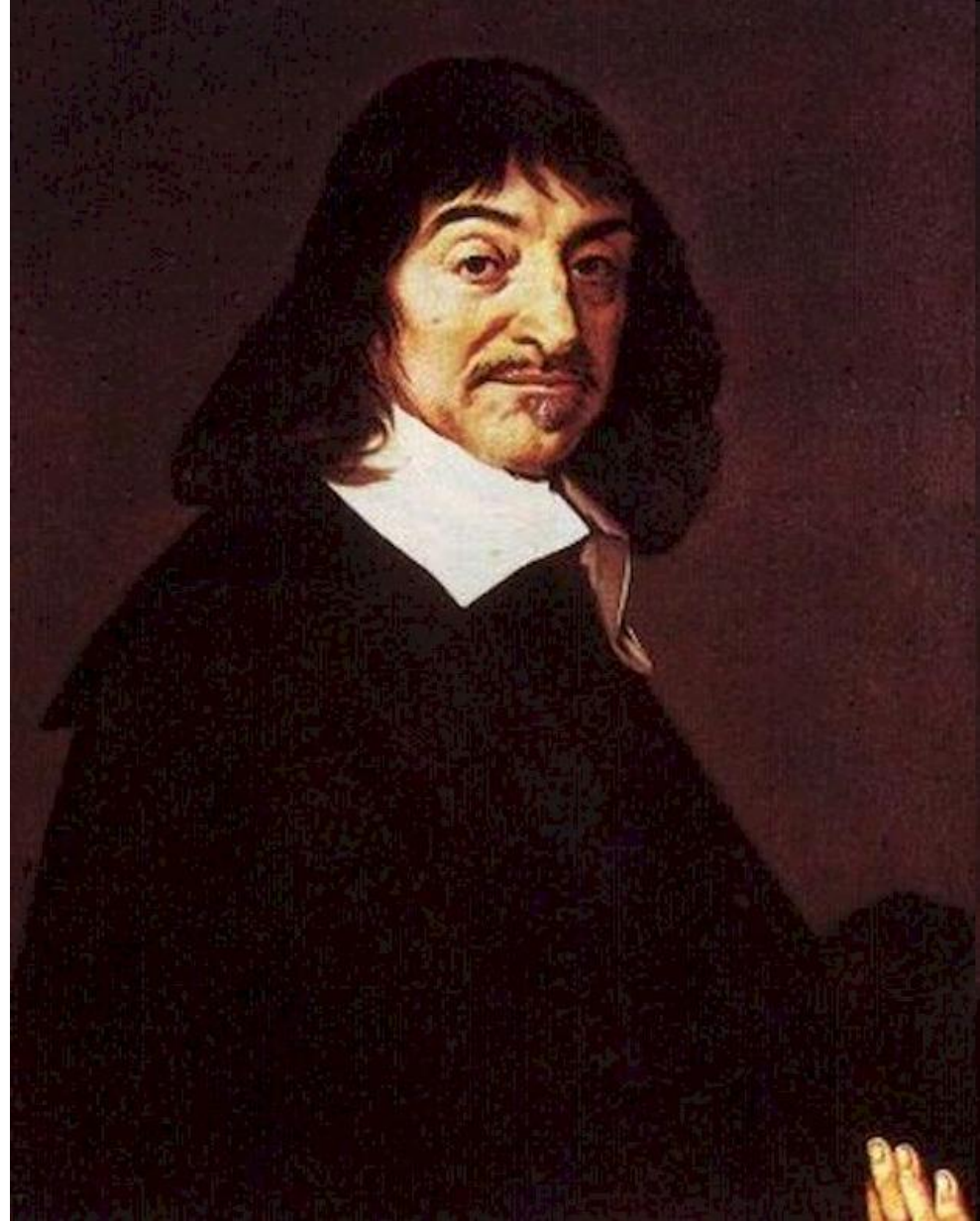
Descartes
